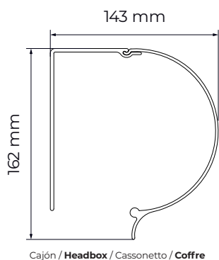
Cajón / Headbox / Cassonetto / Coffre
